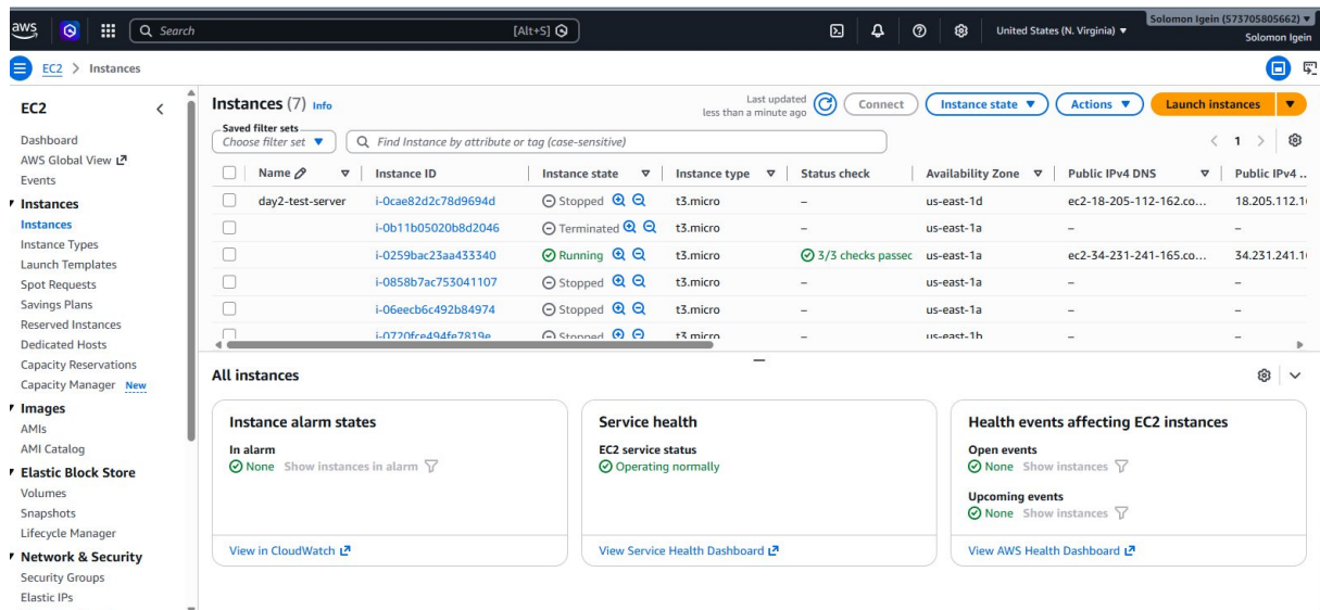
Fig 1: Instances (7) — i-0b11b Terminated → i-0259bac Running 3/3 Promoted from Warm Pool + i-06eeb Refilled — Proof of Chaos Auto-Heal
