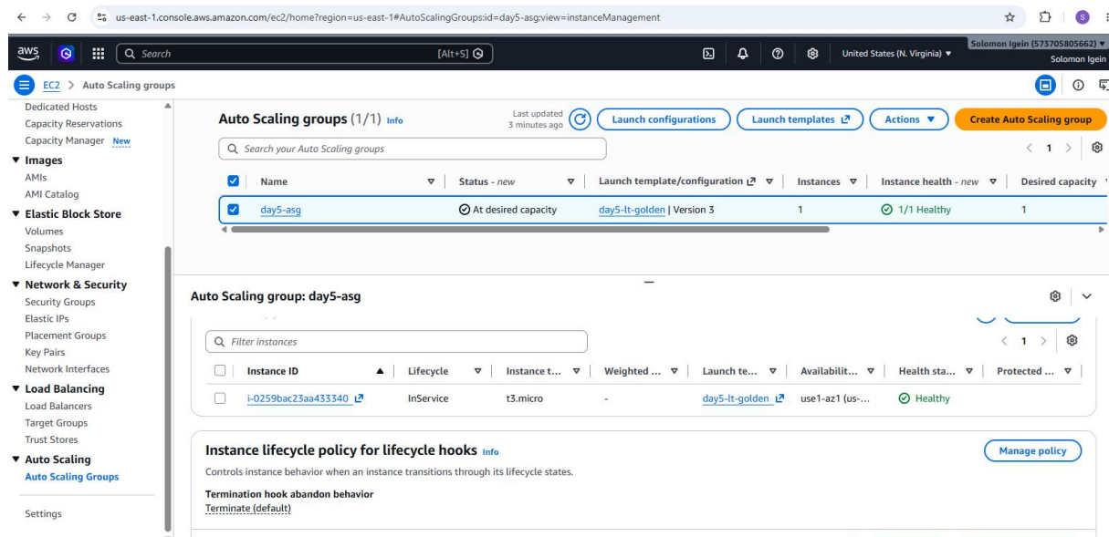
Fig 2: ASG day5-asg At desired capacity Version 3 1/1 Healthy — i-0259bac InService Healthy — After Chaos
