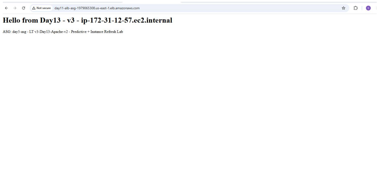
Fig 3: ALB day11-alb-asg-1979065308... → Hello from Day13 - v3 - ip-172-31-12-57.ec2.internal — Zero Downtime After Termination (NEW IP from Warm Pool)
